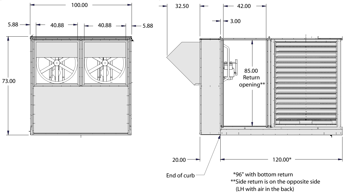
Figure 110: RPS/RFS/RDT 080D to 140D, Side Return Propeller Exhaust Fans (Dimensions in inches)
