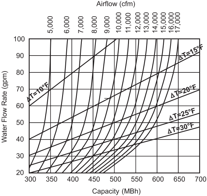
Figure 39: Hot Water Coil, Low Capacity, 015D to 042D
