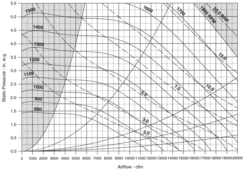
Figure 62: RPS/RFS 035D to 042D 24 in. Airfoil Supply Fan
