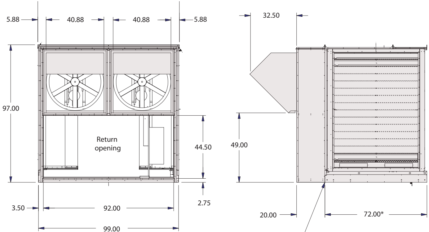
Figure 109: RPS/RFS/RDT 080D to 140D, Back Return Propeller Exhaust Fans (Dimensions in inches)
