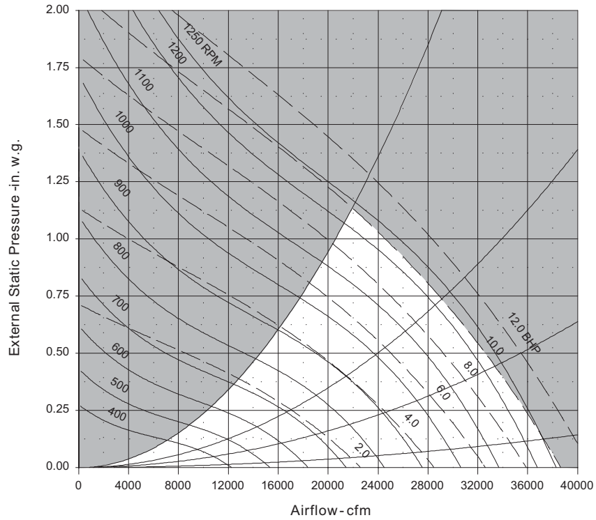
Figure 75: RPS/RFS/RDT 045D to 140D (2) 36 in. Propeller Exhaust Fan
