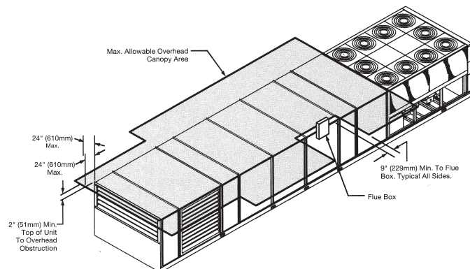
Figure 123: Ventilation Clearances
