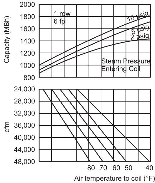
Figure 57: Steam Coil, High Capacity, 080D to 140D
