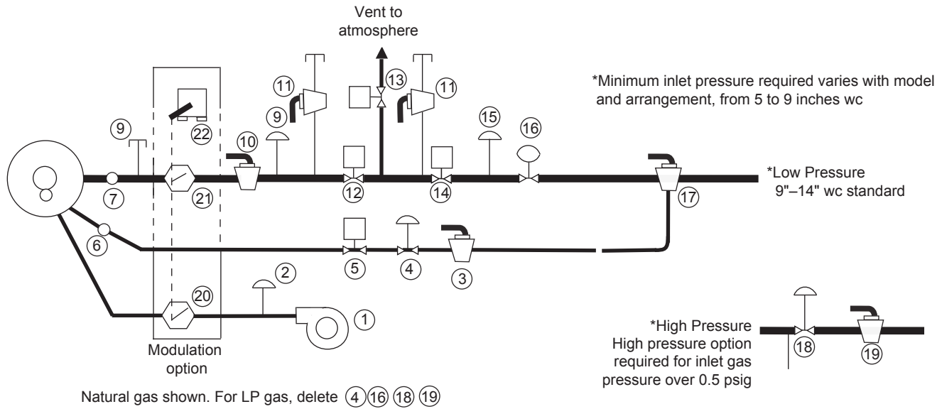
Figure 121: Gas Piping Schematic
