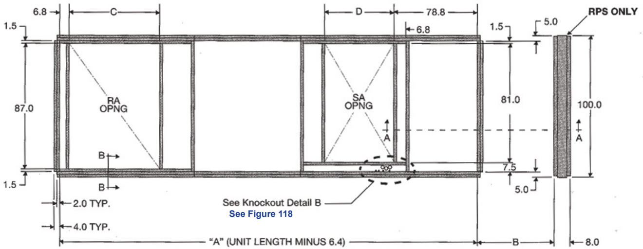
Figure 114: Roof Curb, RPS/RFS/RDT 045D to 140D (with Blank Compartment)
