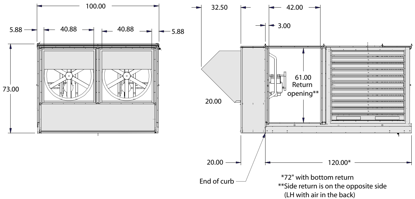
Figure 108: RPS/RFS/RDT 045D to 079D, Side Return Propeller Exhaust Fans (Dimensions in inches)
