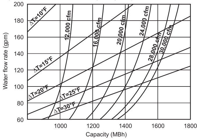
Figure 44: Hot Water Coil, High Capacity, 045D to 079D
