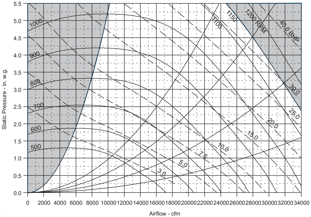
Figure 67: RDT 045D to 079D 40 in. SWSI Airfoil Supply Fan
