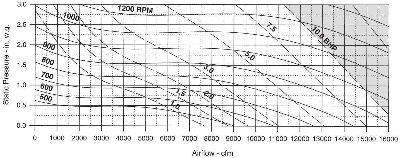
Figure 77: RPS/RFS 015D to 031D, (2) 15 in. x 15 in. Forward Curved Return Fan
