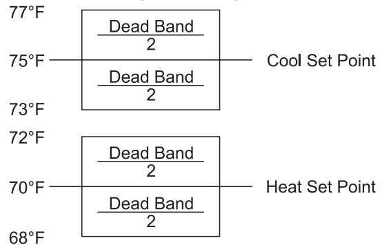
Figure 28: Control Temperature Logic
