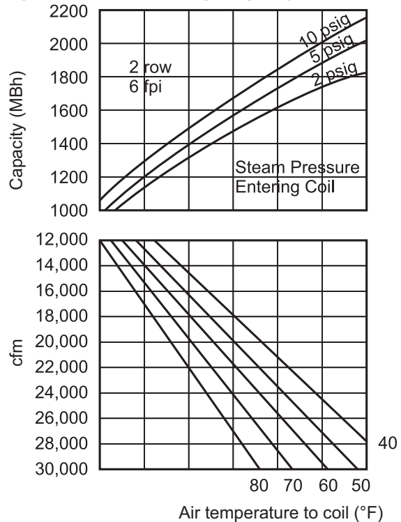
Figure 53: Steam Coil, High Capacity, 045D to 079D
