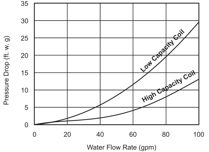
Figure 41: Hot Water Coil Pressure Drop (Headers Included), 015D to 042D
