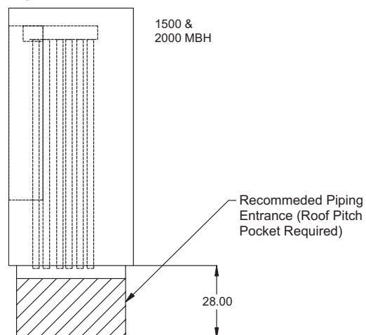
Figure 104: 1500 to 2000 MBh Gas Heat/Heat Section
