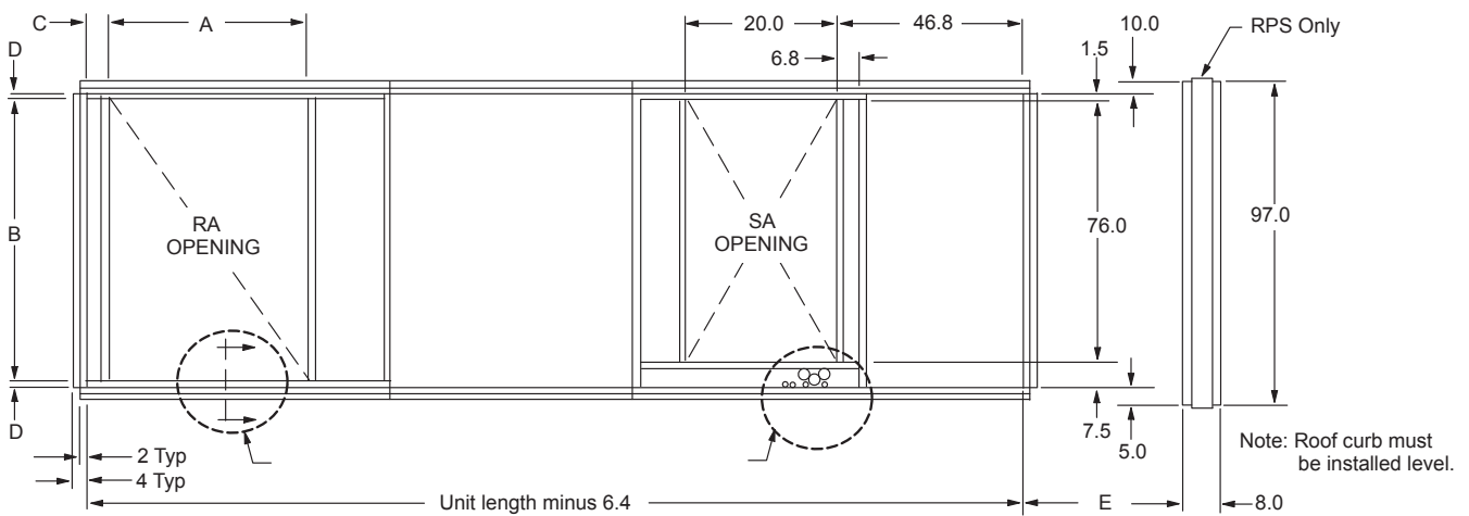
Figure 112: Roof Curb, RPS/RFS/RDT 015D to 042D (with Blank Compartment)
