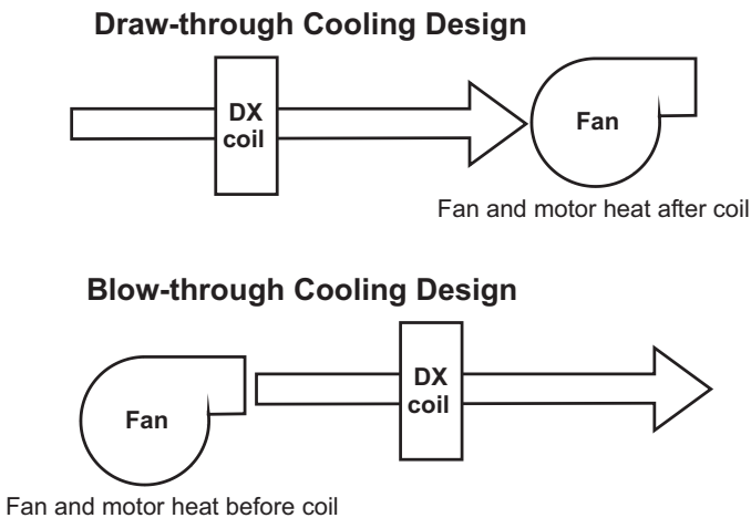
Figure 34: Blow-Through vs. Draw-Through Concept
