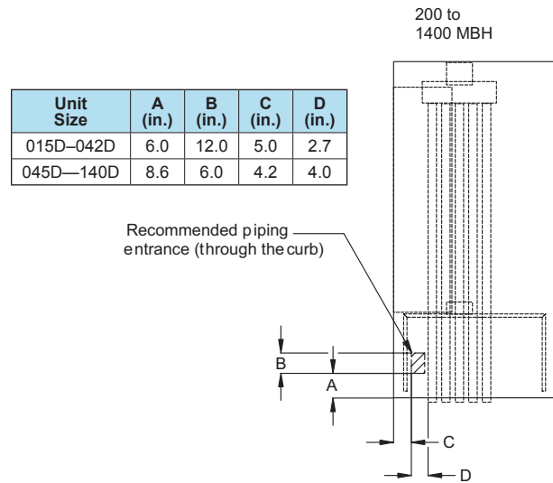
Figure 103: 200 to 1400 MBh Gas Heat/Heat Section
