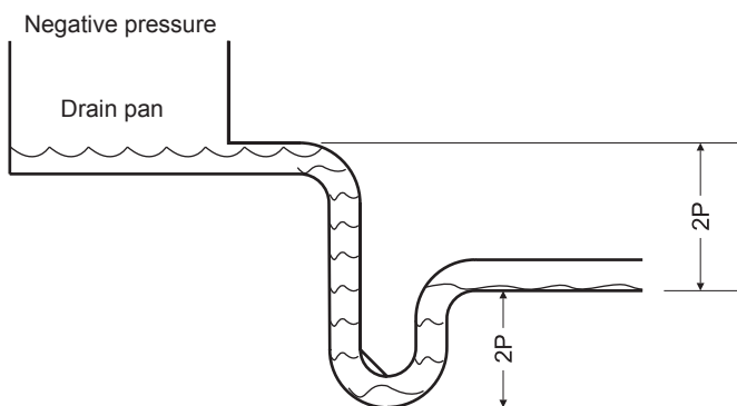
Figure 37: Drain Pan Traps
