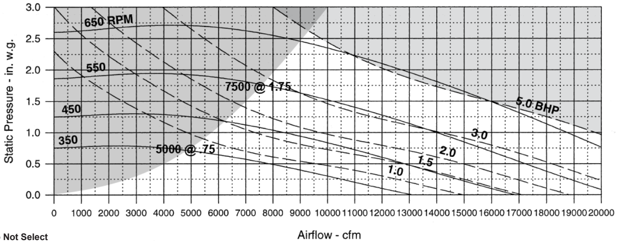
Figure 80: RPS/RFS/RDT 045D to 079D, 40 in. SWSI Airfoil Return Fan
