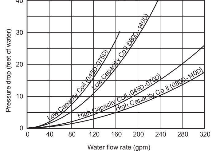
Figure 47: Hot Water Coil Pressure Drop (headers included, does not include valve and valve piping), 045D to 140D
