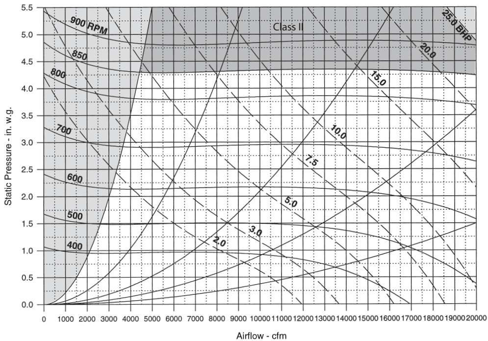
Figure 61: RPS/RFS 035D to 042D 24 in. Forward Curve Supply Fan
