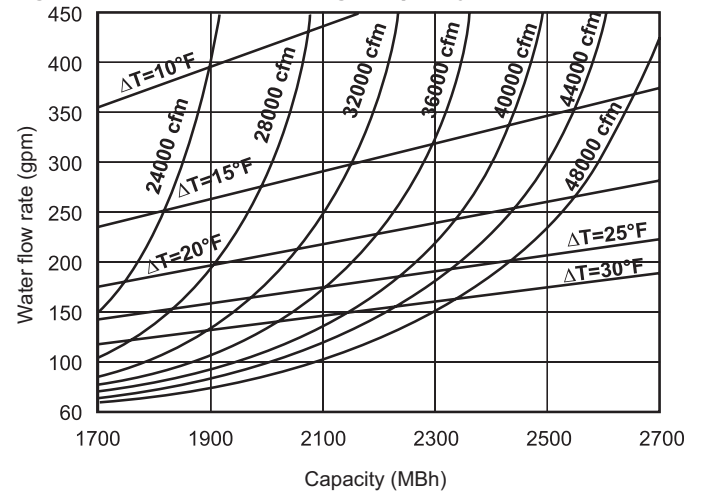
Figure 46: Hot Water Coil, High Capacity, 080D to 140D
