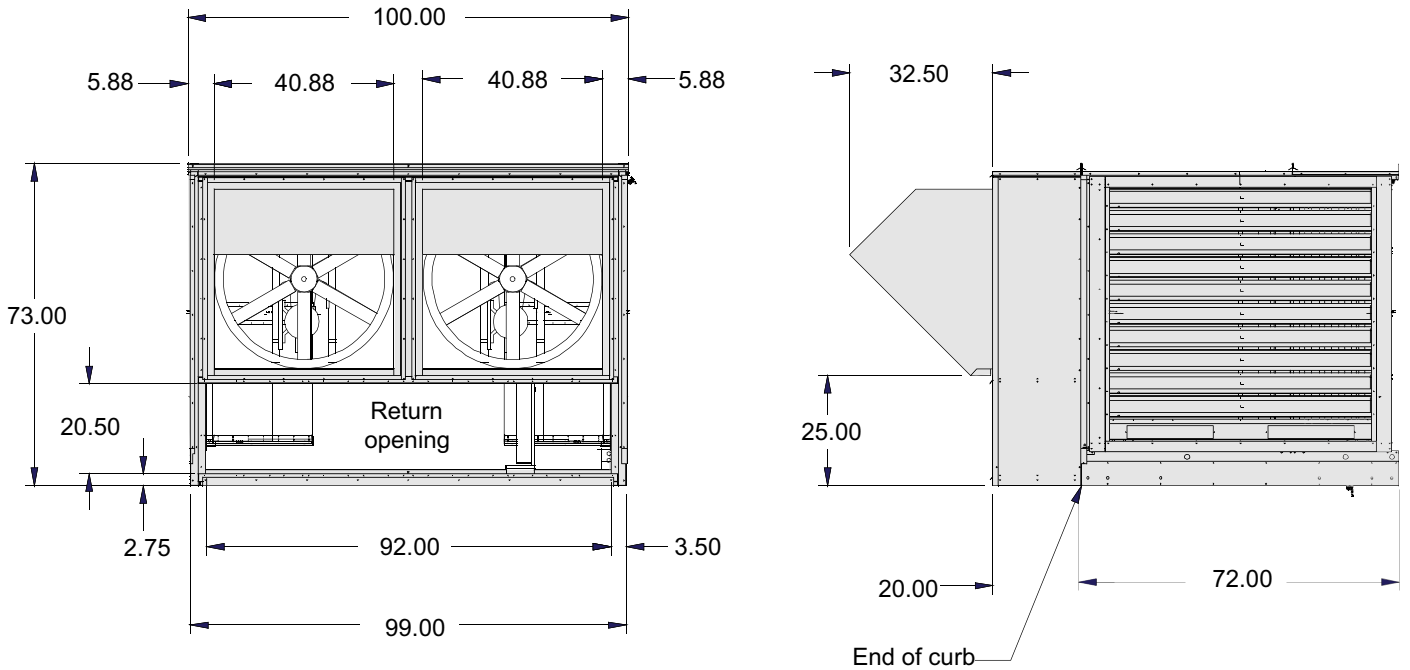
Figure 107: RPS/RFS/RDT 045D to 079D, Back Return Propeller Exhaust Fans (2 Shown, Dimensions in inches)
