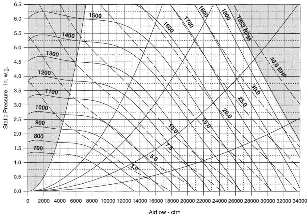
Figure 64: RPS/RFS 045D to 050D 27 in. Airfoil Supply Fan
