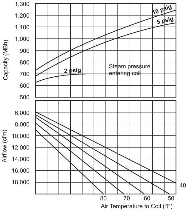
Figure 51: Steam Coil, High Capacity, 015D to 042D
