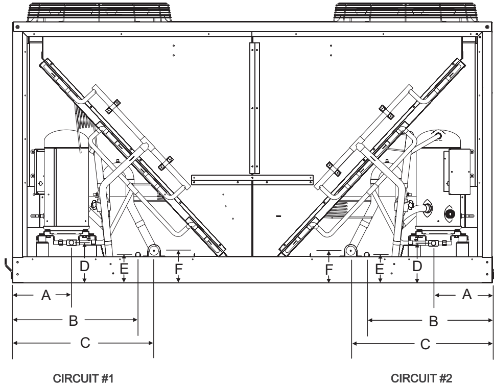
Figure 120: Refrigerant Piping Connection Locations Example
