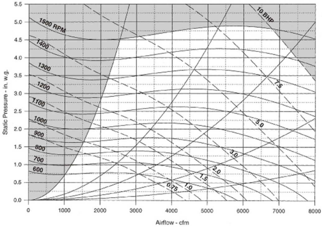
Figure 58: RPS/RFS 015D to 031D (2) 15 in. × 6 in. Forward Curved Supply Fan
