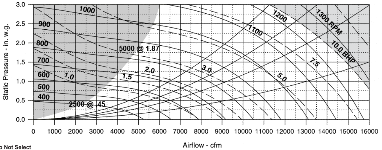
Figure 81: RPS/RFS/RDT 080D to 140D, 44 in. SWSI Airfoil Return Fan
