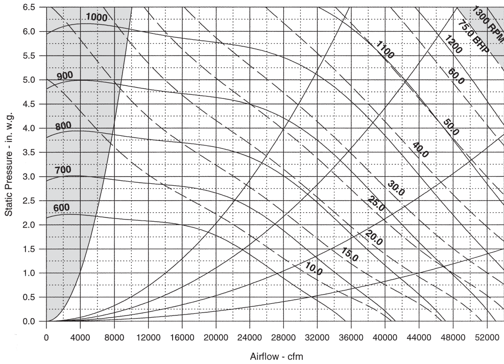
Figure 73: RPS/RFS 080D to 140D 40 in. Airfoil Supply Fan
