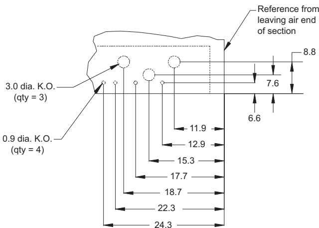
Figure 100: Main Control Panel/Discharge Plenum, RPS/RFS/RDT 045D to 140D
