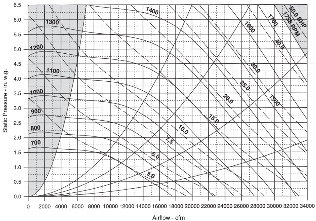
Figure 65: RPS/RFS 045D to 079D 30 in. Airfoil Supply Fan
