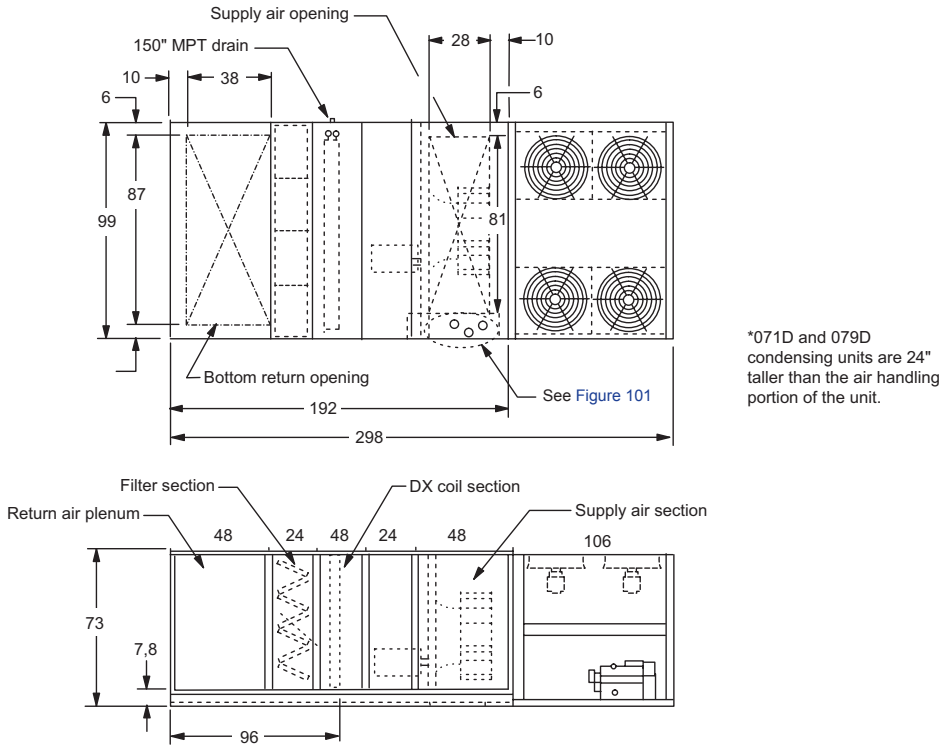
Figure 97: RDT 070D to 079D
