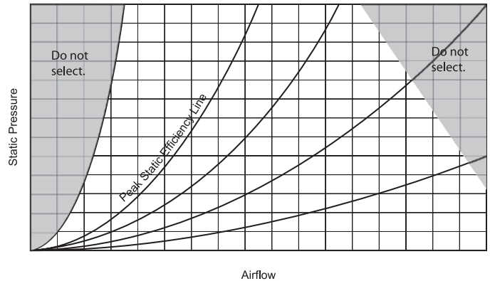
Figure 31: Optimal Fan Selection Line
