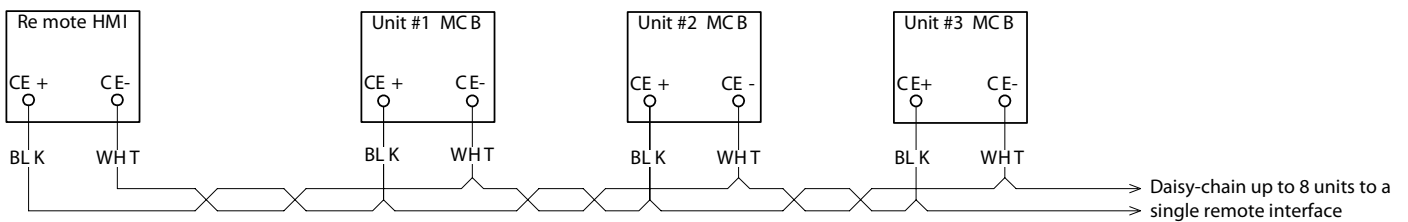
Figure 25: Process Bus Wiring Connections
