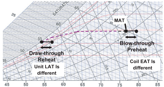
Figure 35: Blow-Through vs. Draw-Through Performance
