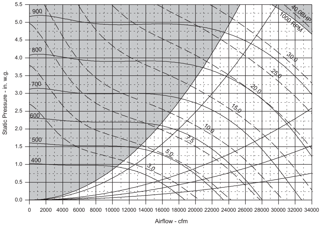
Figure 68: RDT 045D to 079D 44 in. SWSI Airfoil Supply Fan
