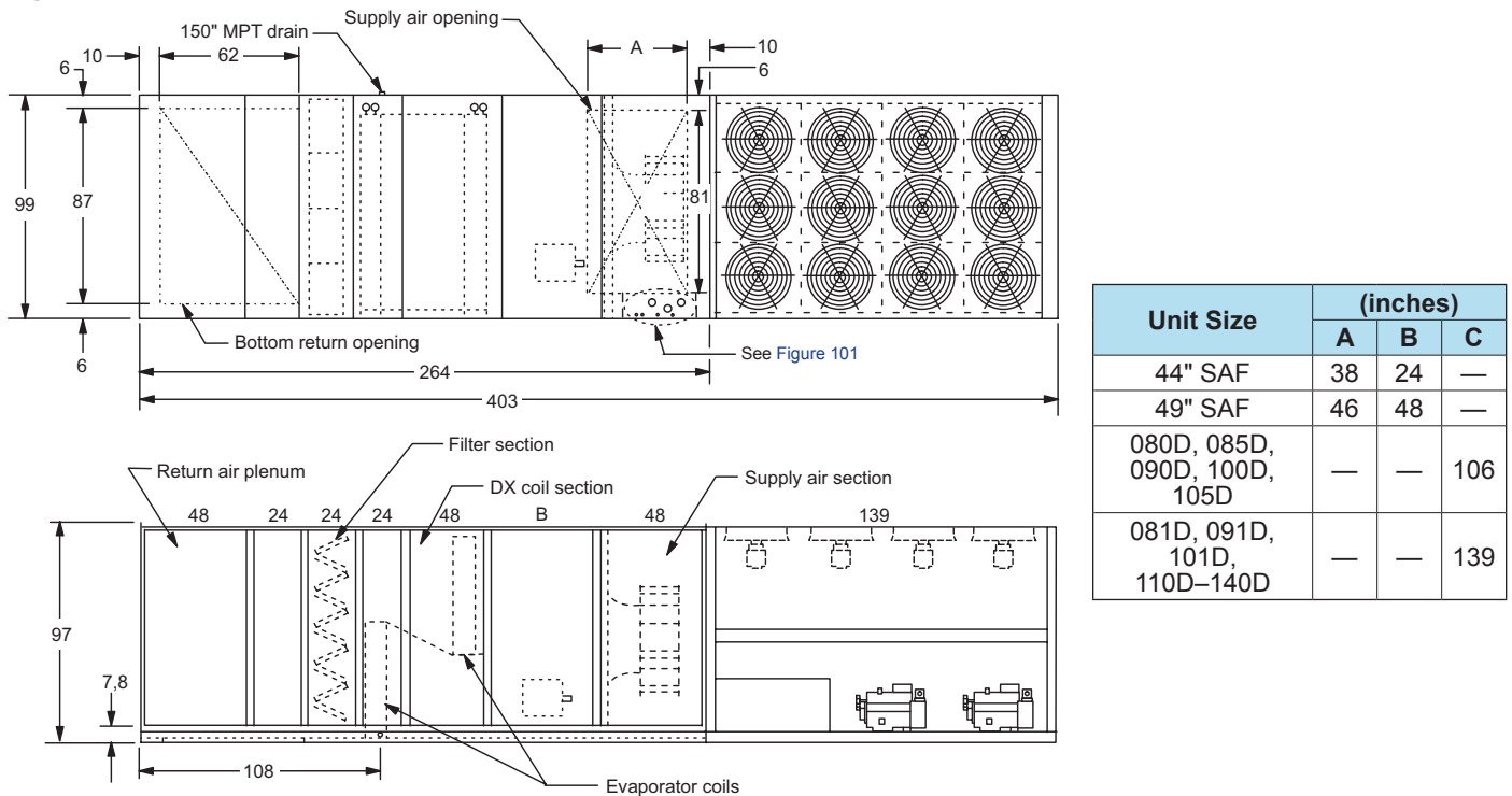
Figure 98: RDT 080D to 140D
