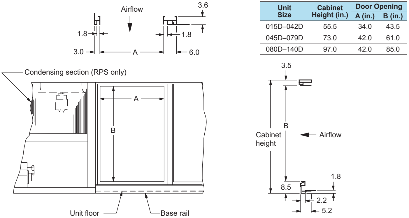
Figure 105: Side Discharge
