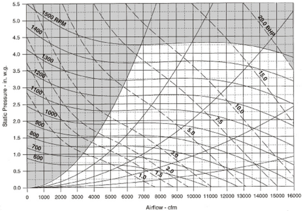
Figure 59: RPS/RFS 015D to 031D (2) 15 in. × 15 in. Forward Curved Supply Fan
