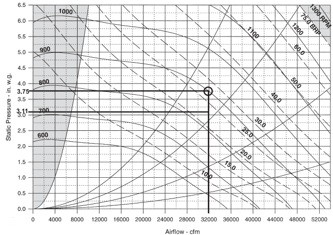
Figure 36: RPS 105C to 135C 40" DWDI Airfoil
