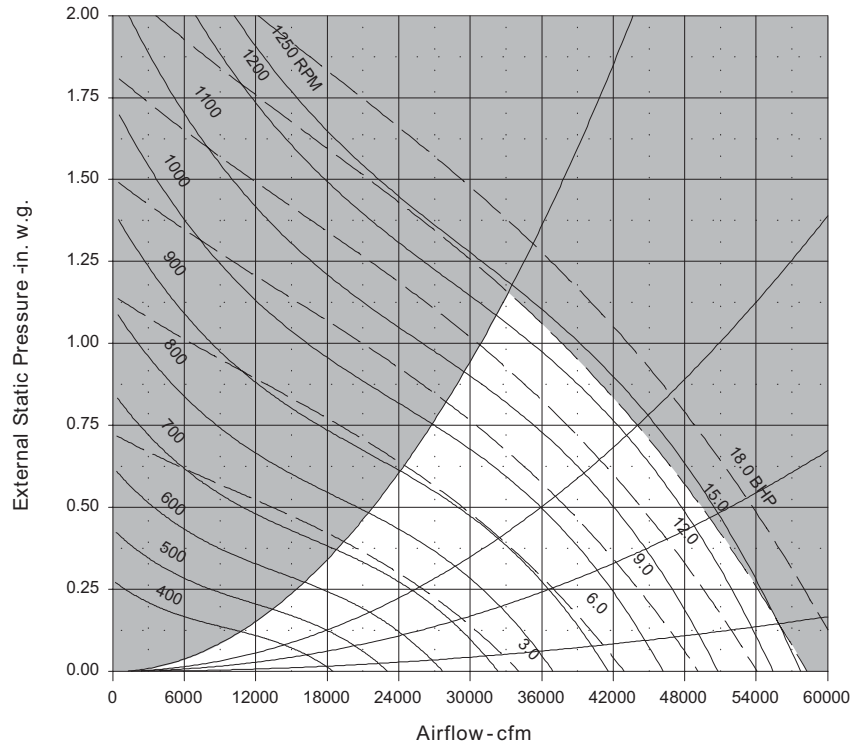
Figure 76: RPS/RFS/RDT 080D to 140D (3) 36 in. Propeller Exhaust Fan
