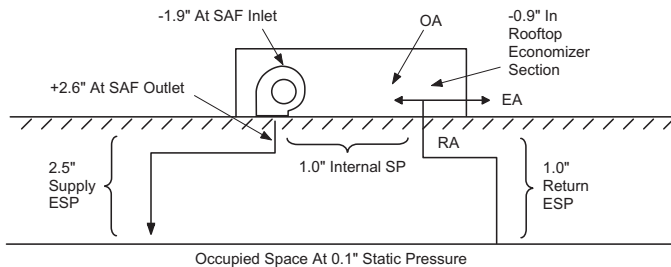
Figure 32: Supply Air Fan Only System Static Pressures with 1" Return Duct ESP
