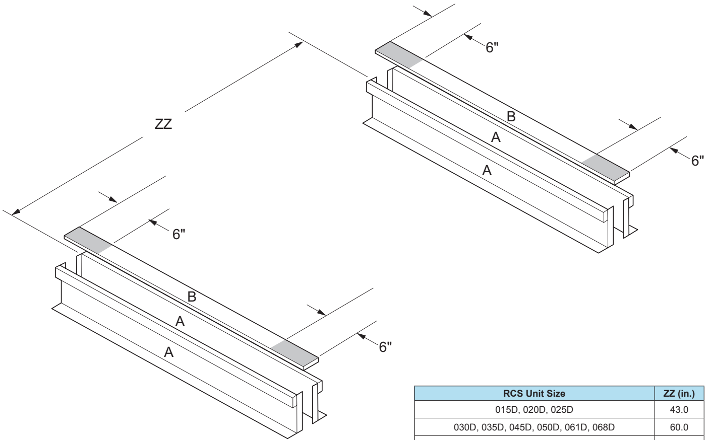
Figure 119: RCS Roof Installation
