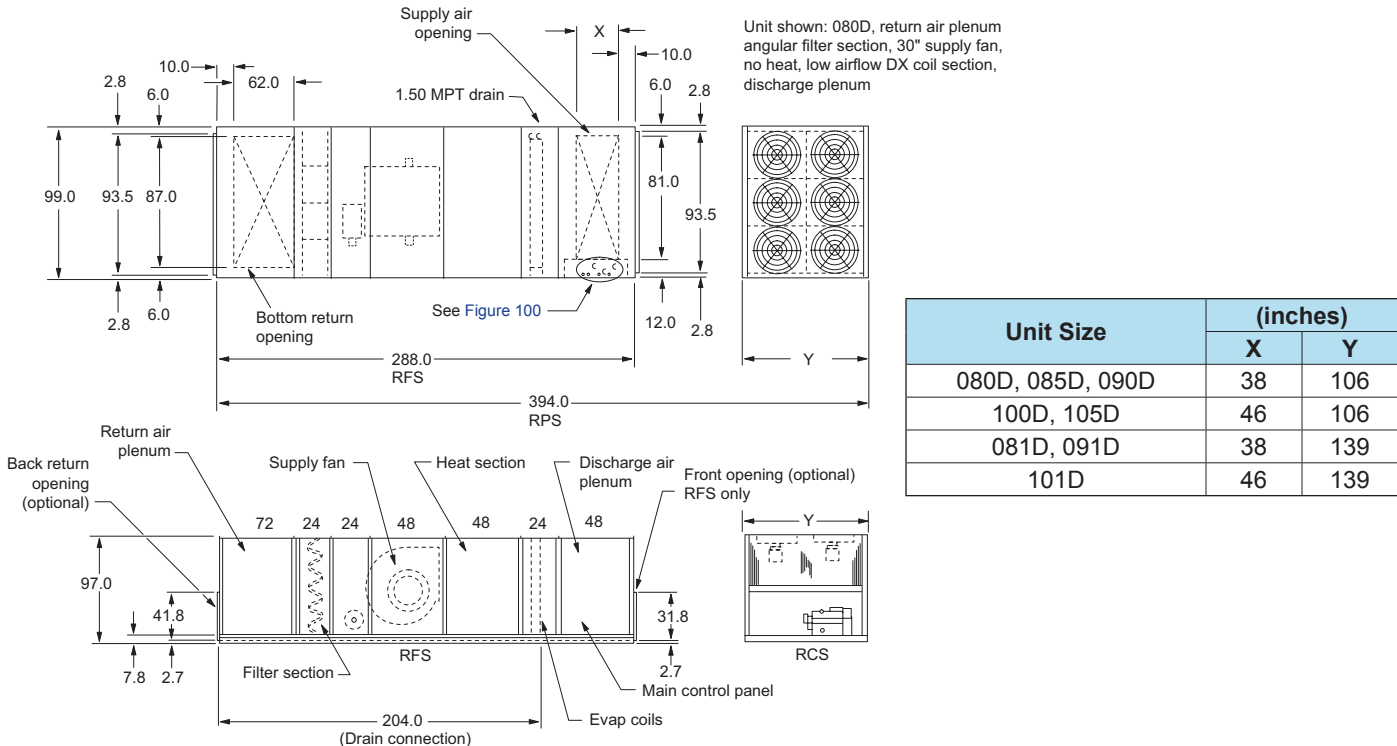
Figure 94: RPS/RFS/RCS 080D to 105D
