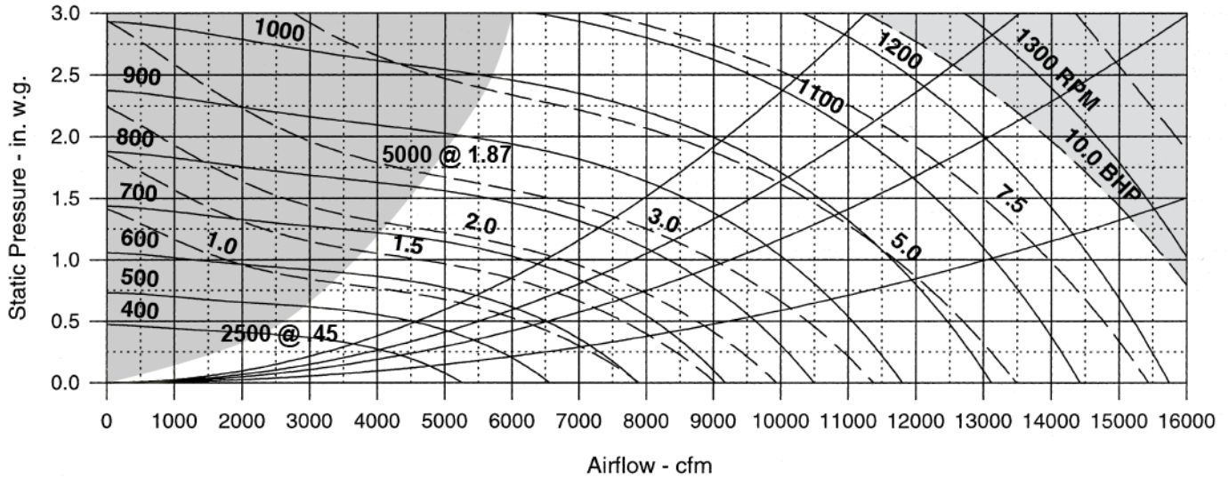
Figure 78: RPS/RFS 015D to 042D, 30 in. SWSI Airfoil Return Fan*
