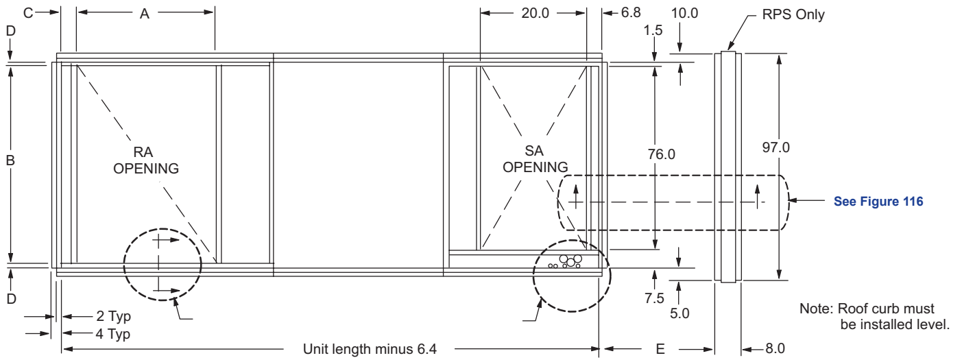
Figure 111: Roof Curb, RPS/RFS/RDT 015D to 042D (without Blank Compartment)
