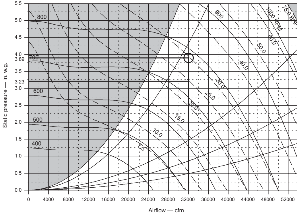
Figure 70: RDT 080D to 140D 49 in. SWSI Airfoil Supply Fan
