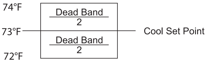
Figure 29: Compressorized Logic
