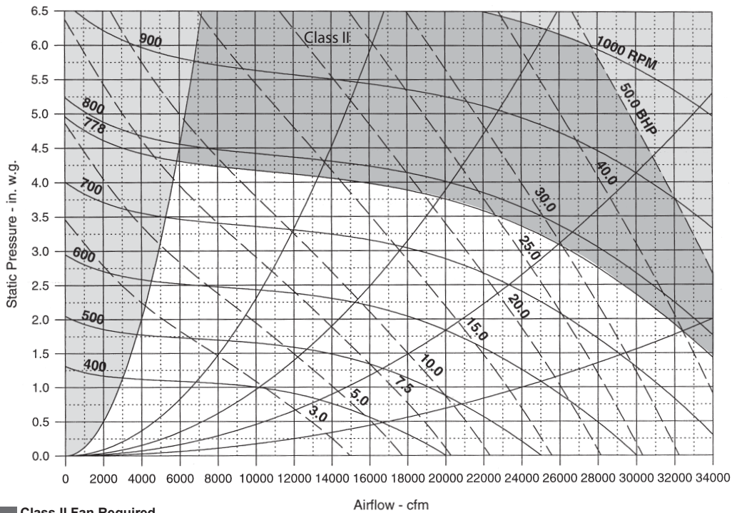
Figure 63: RPS/RFS 045D to 050D 27 in. Forward Curved Supply Fan
