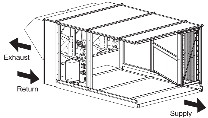
Figure 16: Airflow Configuration—Exhaust Fan
