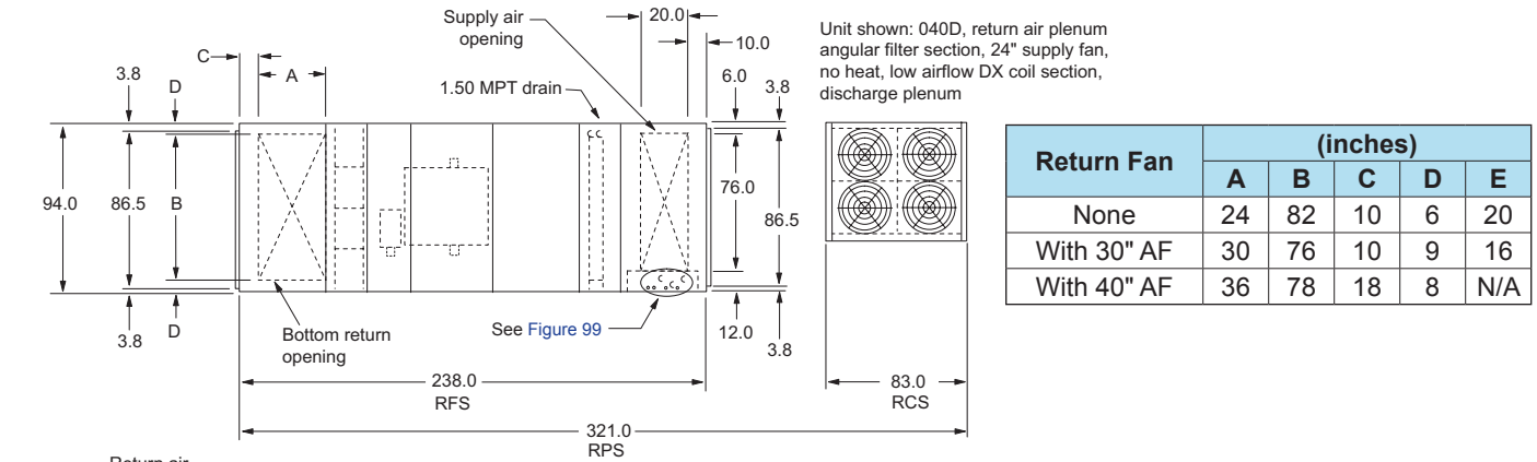
Figure 92: RPS/RFS/RCS 035D to 042D, Basic Configuration
