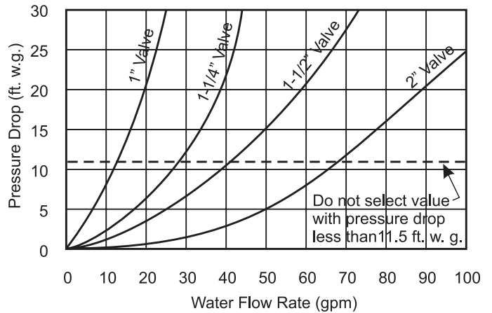
Figure 42: Hot Water Valve and Piping Pressure Drop, 015D to 042D
