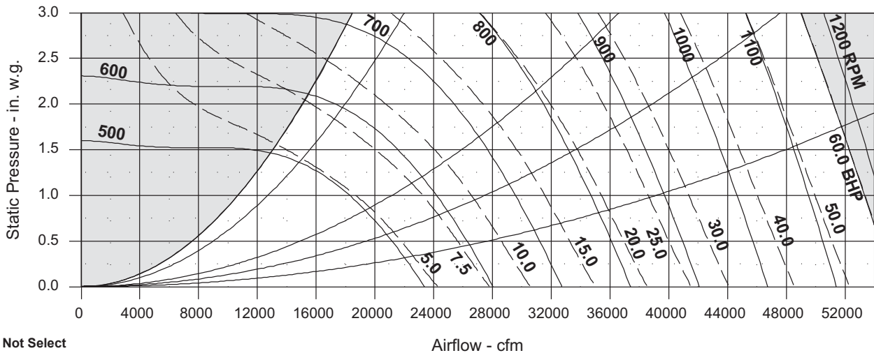
Figure 81: RPS/RFS/RDT 080D to 140D, 44 in. SWSI Airfoil Return Fan
