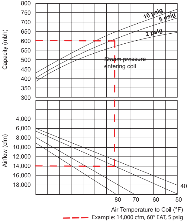
Figure 50: Steam Coil, Low Capacity, 015D to 042D
