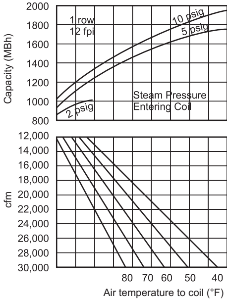
Figure 55: Steam Coil, Medium Capacity, 080D to 140D
