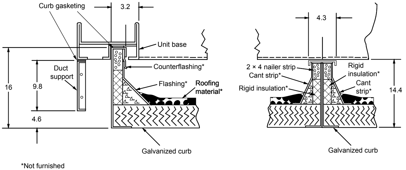
Figure 116: Curb Cross Section
