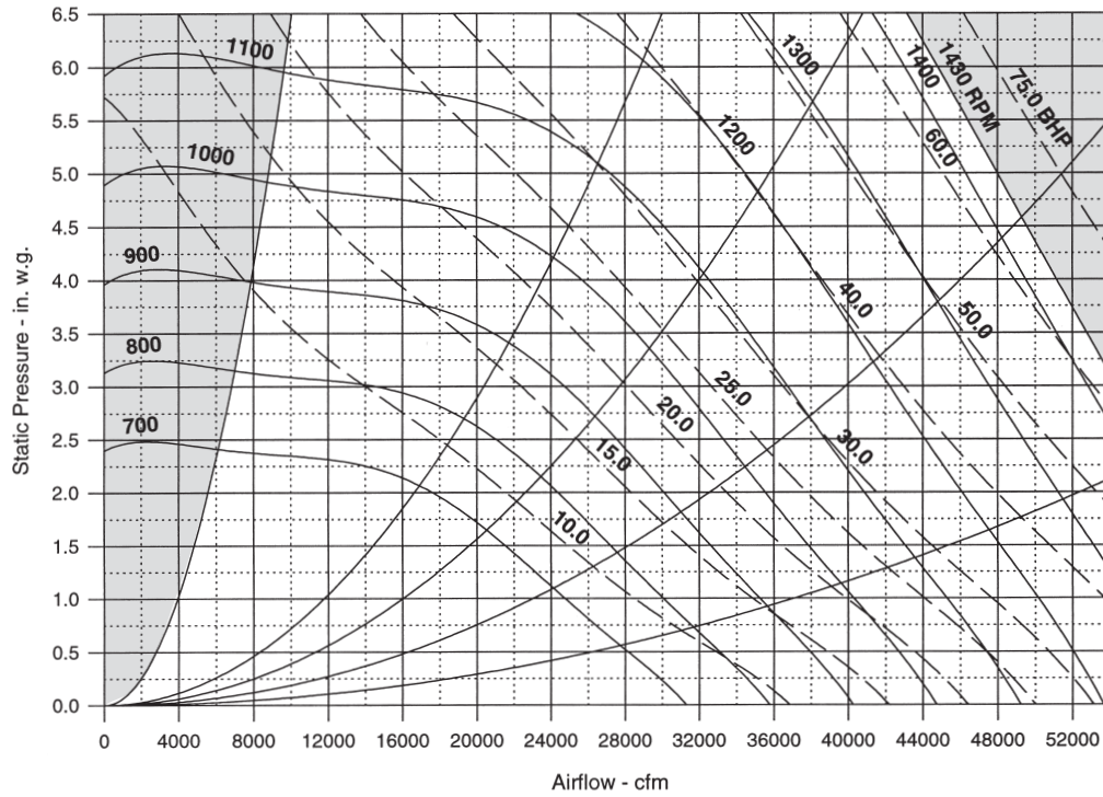
Figure 72: RPS/RFS 080D to 140D 36 in. Airfoil Supply Fan
