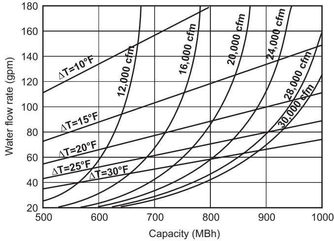
Figure 43: Hot Water Coil, Low Capacity, 045D to 079D
