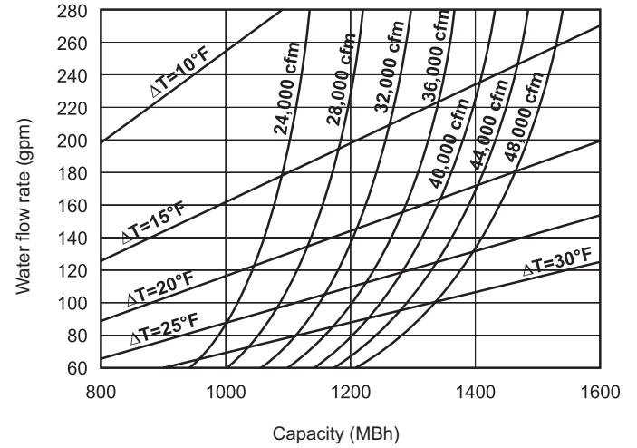
Figure 45: Hot Water Coil, Low Capacity, 080D to 140D
