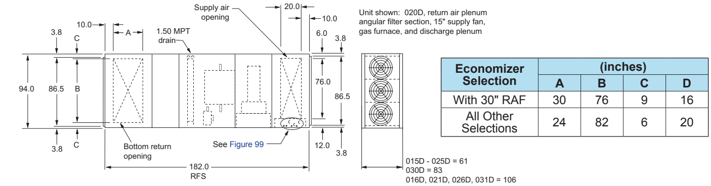
Figure 91: RPS/RFS/RCS 015D to 031D, Basic Configuration
