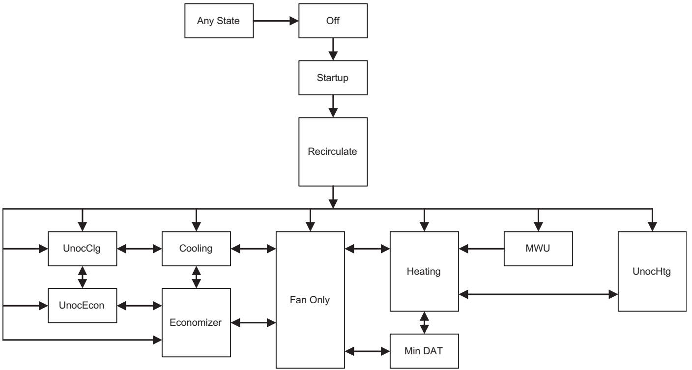
Figure 30: Operating State Sequence Chart
