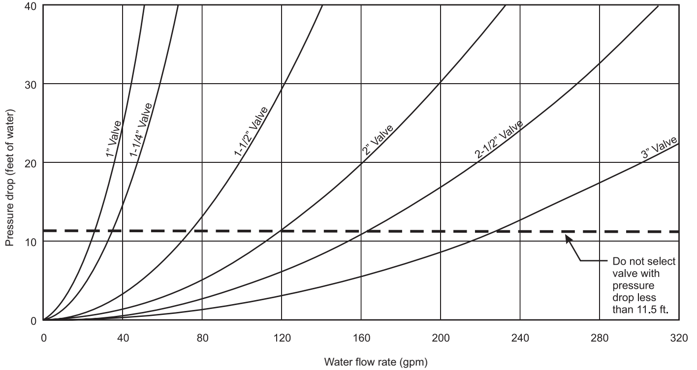
Figure 48: Hot Water Valve Pressure Drop (does not include piping and coil), RPS and RFS 045D to 140D
