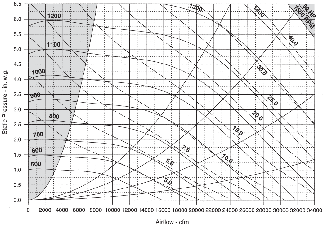
Figure 66: RPS/RFS 060D to 079D 33 in. Airfoil Supply Fan
