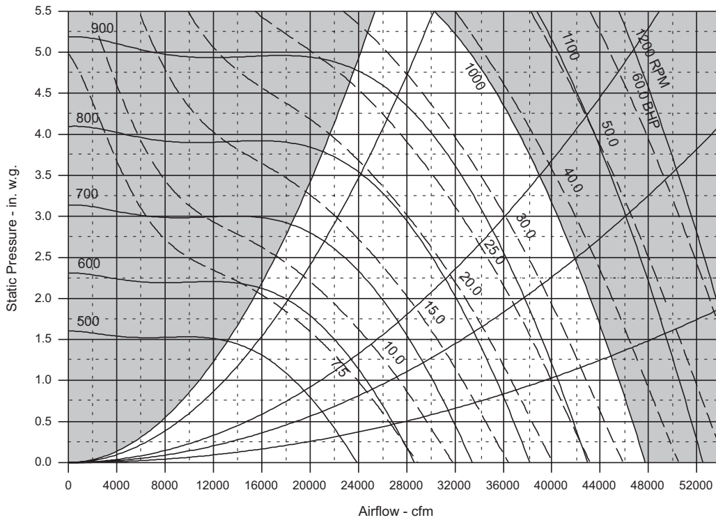
Figure 69: RDT 080D to 140D 44 in. SWSI Airfoil Supply Fan
