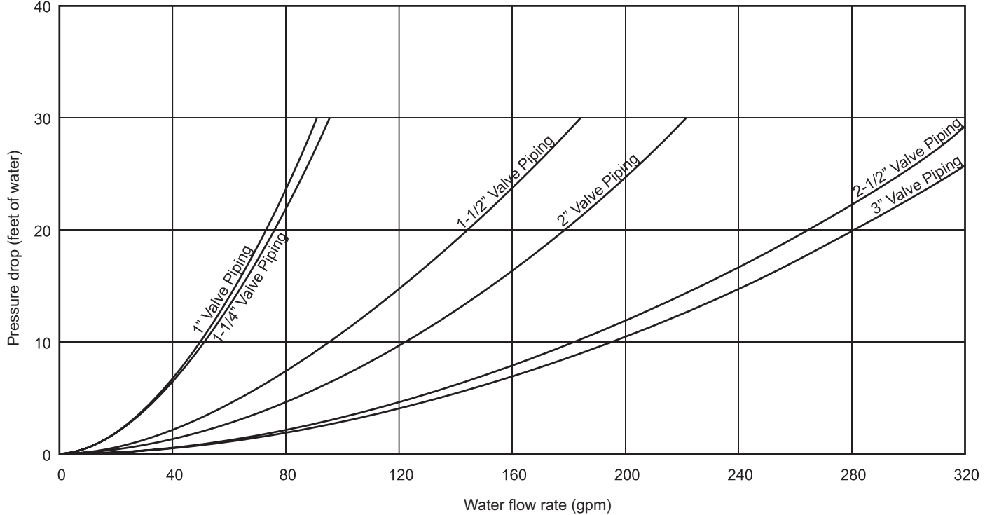
Figure 49: Hot Water Piping Pressure Drop (does not include valve and coil), RPS and RFS 045D to 140D
