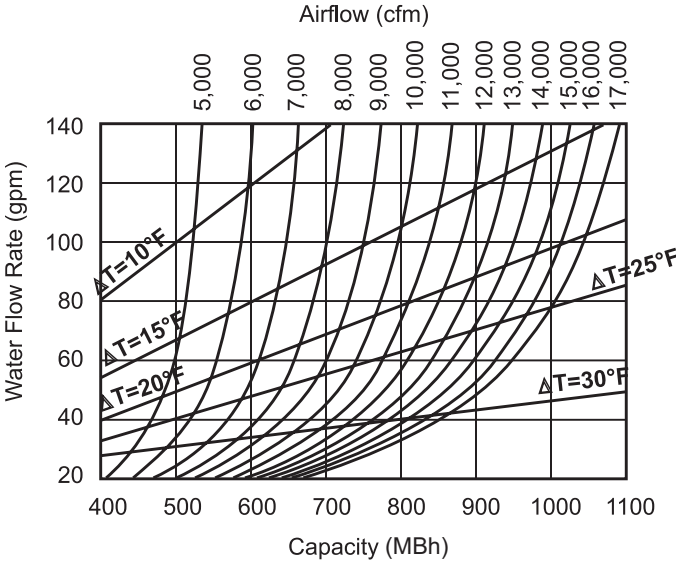
Figure 40: Hot Water Coil, High Capacity, 015D to 042D
