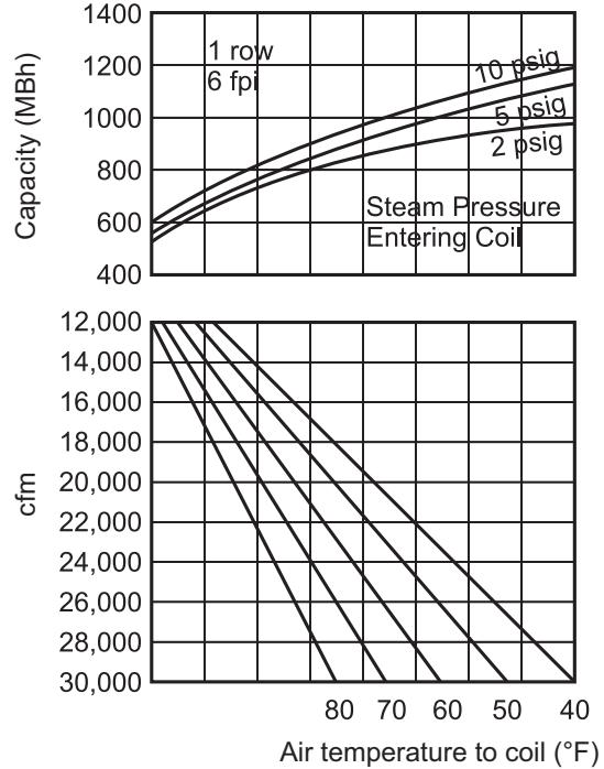
Figure 52: Steam Coil, Low Capacity, 045D to 079D
