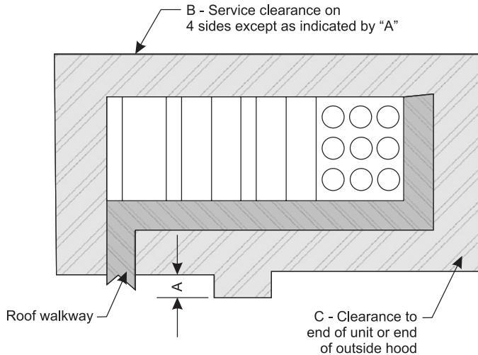
Figure 122: Service Clearances
