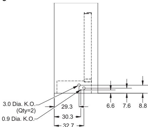
Figure 101: Electric Heat/Heat Section
