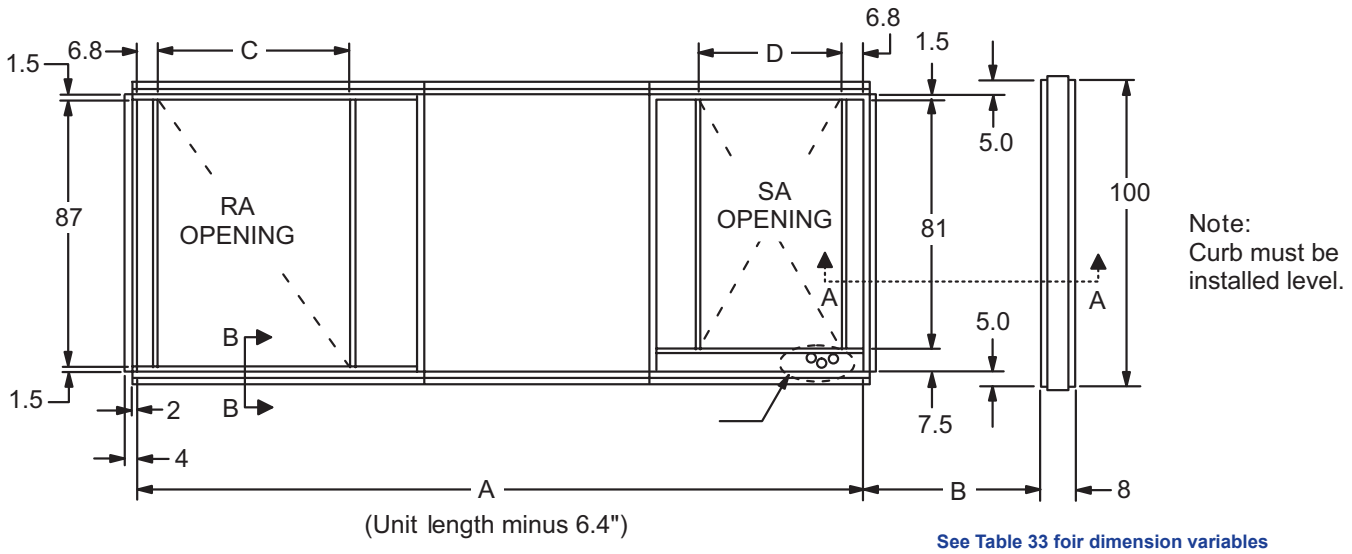
Figure 113: Roof Curb, RPS/RFS/RDT 045D to 140D (without Blank Compartment)
