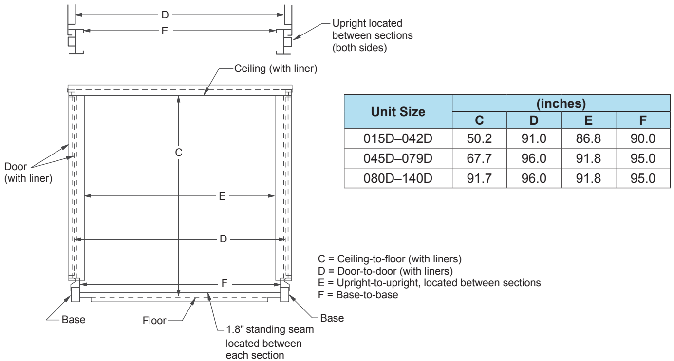
Figure 106: Internal Cabinet Clearance, Air Toward Face
