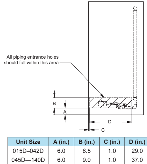
Figure 102: Steam and Hot Water Heat/Heat Section
