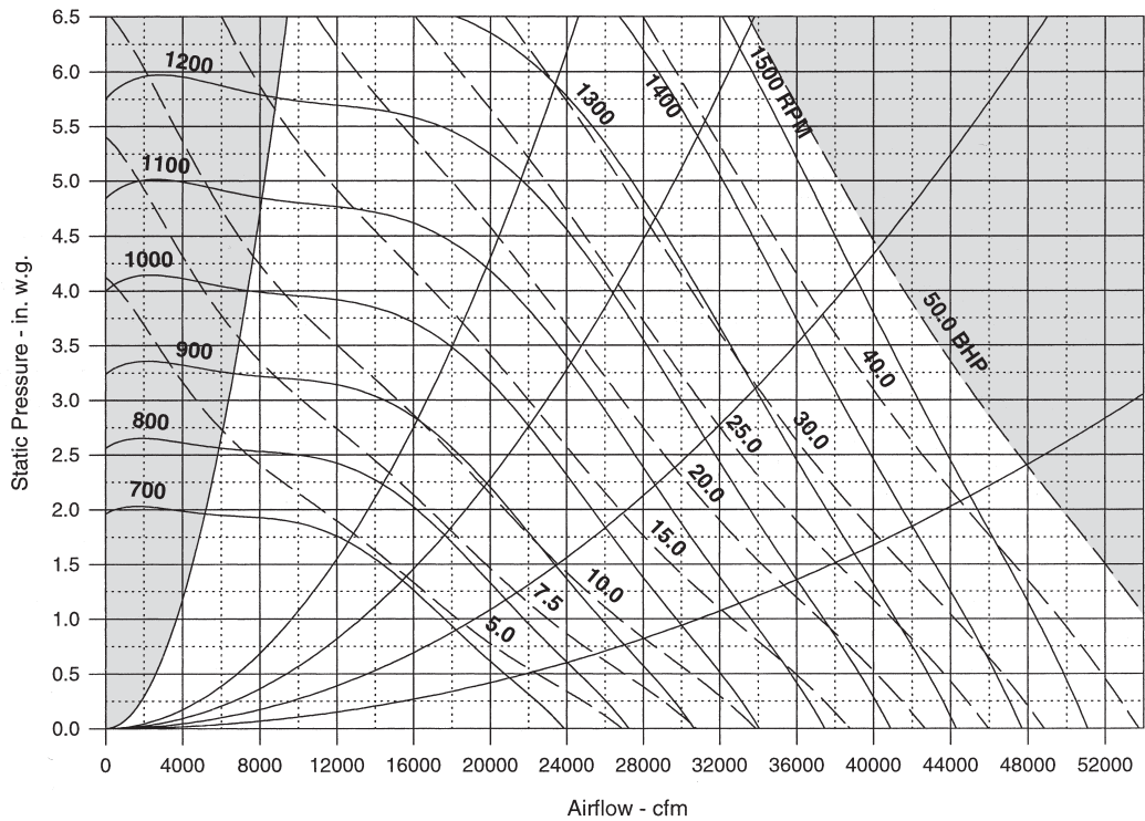
Figure 71: RPS/RFS 080D to 105D 33 in. Airfoil Supply Fan
