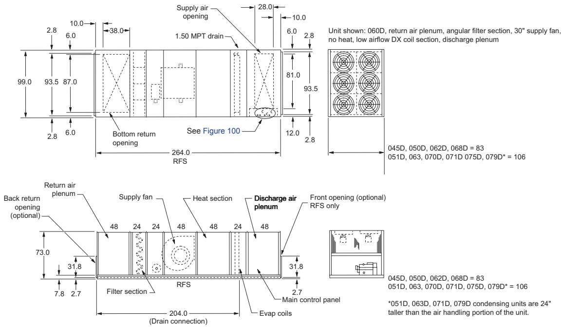
Figure 93: RPS/RFS/RCS 045D to 079D
