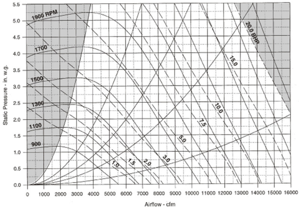
Figure 60: RPS/RFS 015D to 031D 20 in. Airfoil Supply Fan
