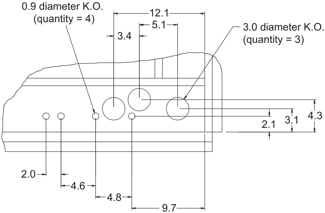
Figure 118: Knockout Detail, 045D to 140D
