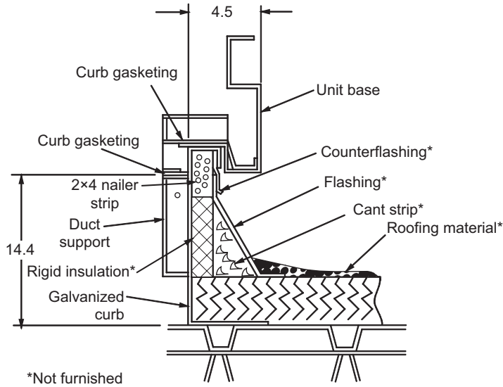
Figure 115: Curb Cross Section
